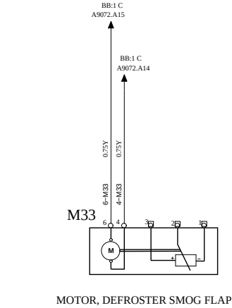
MOTOR, DEFROSTER SMOG FLAP
