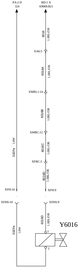
ROOF VALVE, REHEATING SYSTEM
